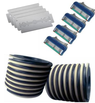
Wendt Product – Resin Bond Wheels
